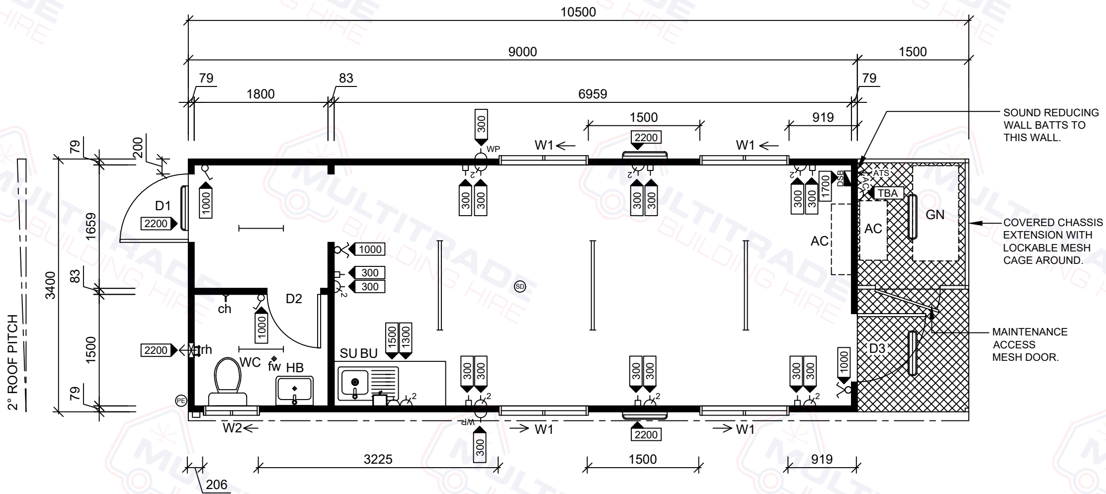
10.5x3.4m Gatehouse - Floor Plan
